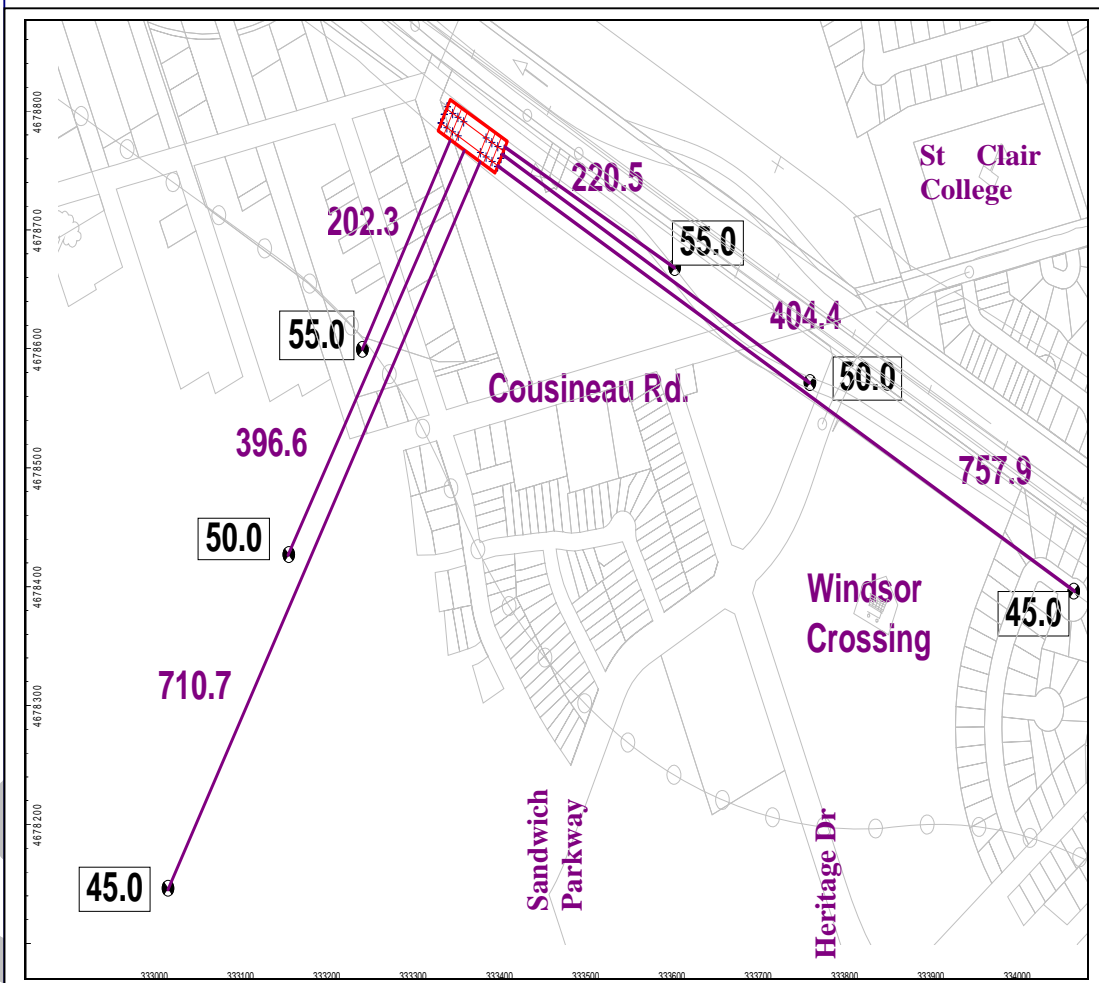
FIGURE 5.2-1 SEPARATION DISTANCES (M) FOR OPTION 1A – VENTILATION BUILDING – NO MITIGATION
